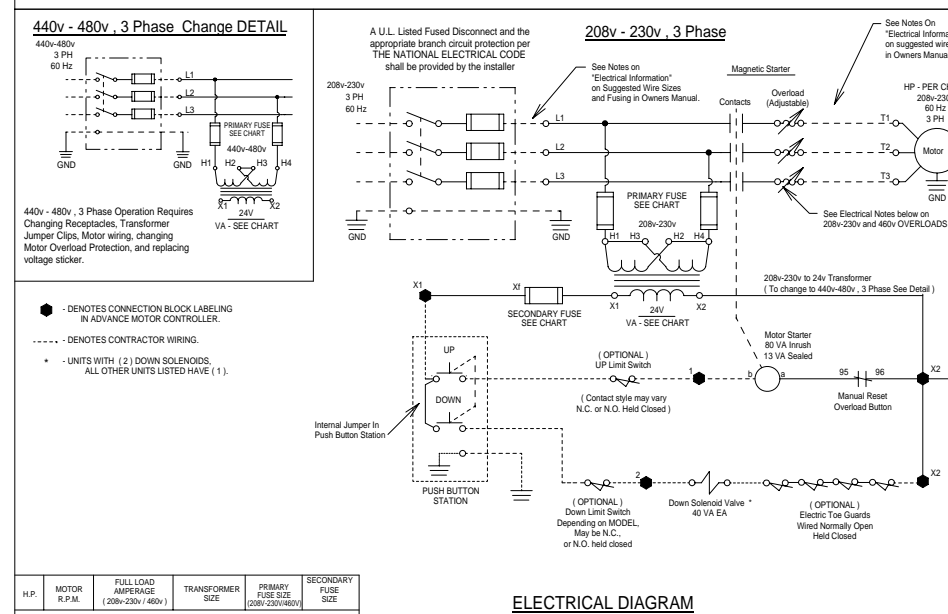
ELECTRICAL DIAGRAM
