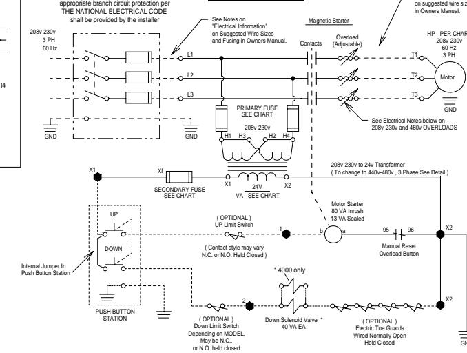
ELECTRICAL DIAGRAM
