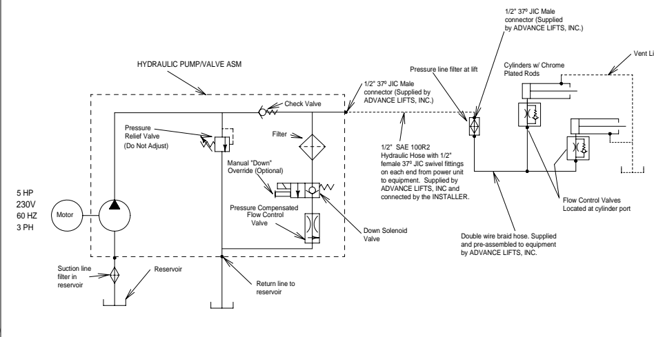
HYDRAULIC DIAGRAM
