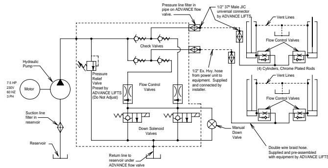
HYDRAULIC DIAGRAM
